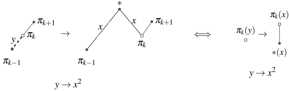
Figure 10: y is on the rise.
