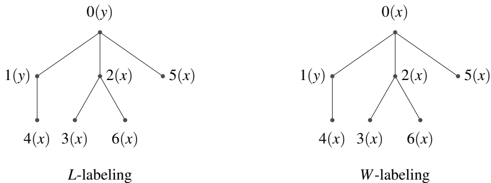
Figure 15: Two labelings of an increasing tree.
