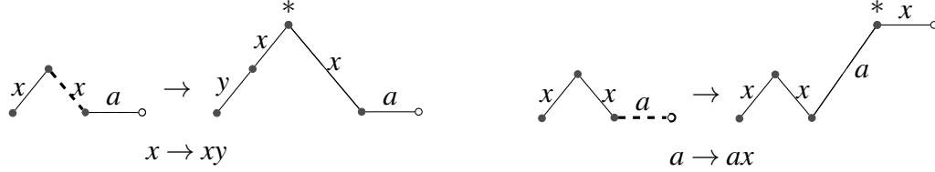
Figure 3: The labeling of \sigma ends with xa .
