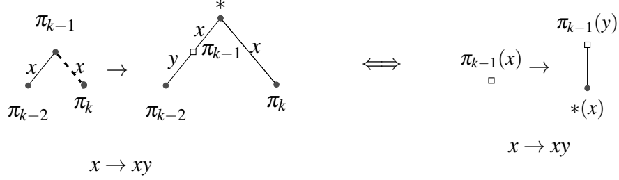
Figure 9: x is on the fall.
