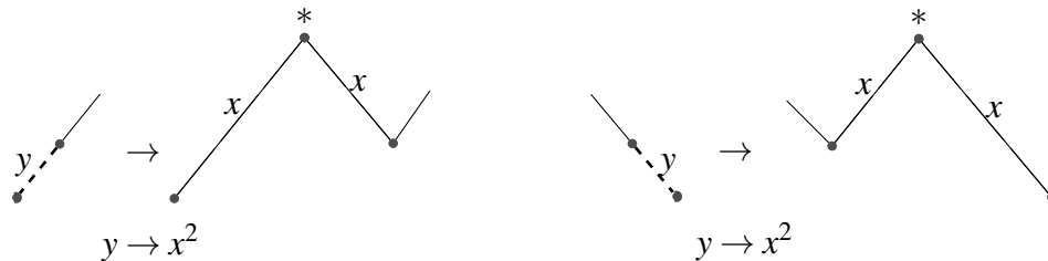
Figure 2: Insertion at a position labeled by y .
