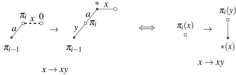
Figure 13: The case k = i + 1 and \pi_{i-1} < \pi_i .
