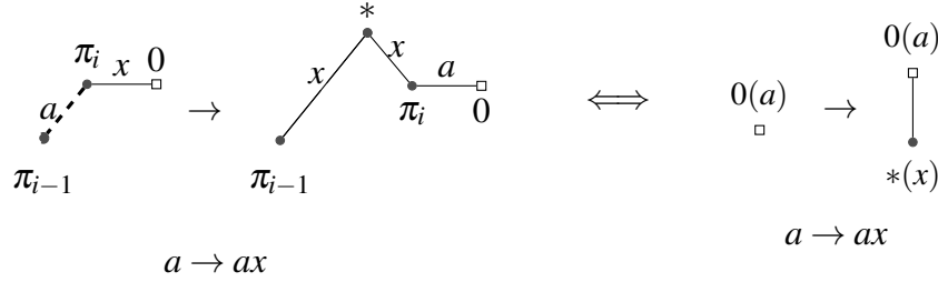
Figure 12: The case k = i and \pi_{i-1} < \pi_i .
