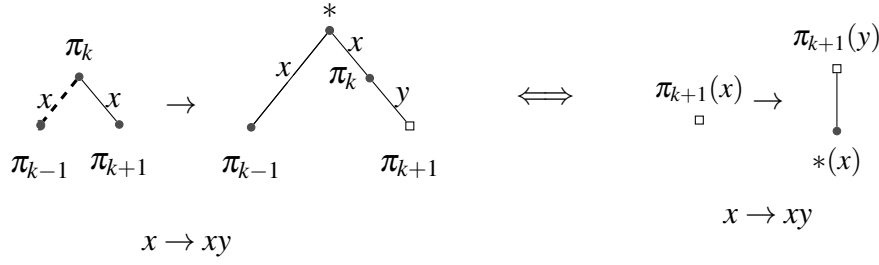
Figure 8: x is on the rise.
