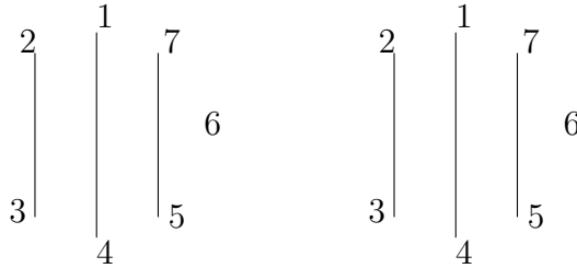
Figure 5: The canonical spanning tree
