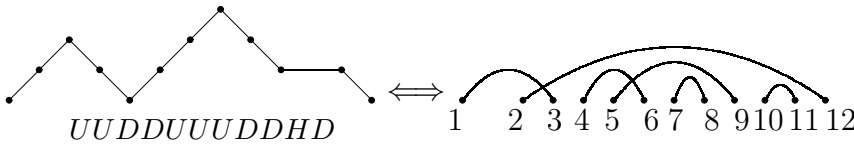
Figure 7. The bijection \phi .
